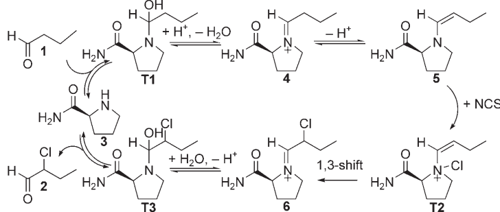
Scheme 2. Proposed mechanism of the L-prolinamide-catalyzed \alpha -chlorination of butanal.
