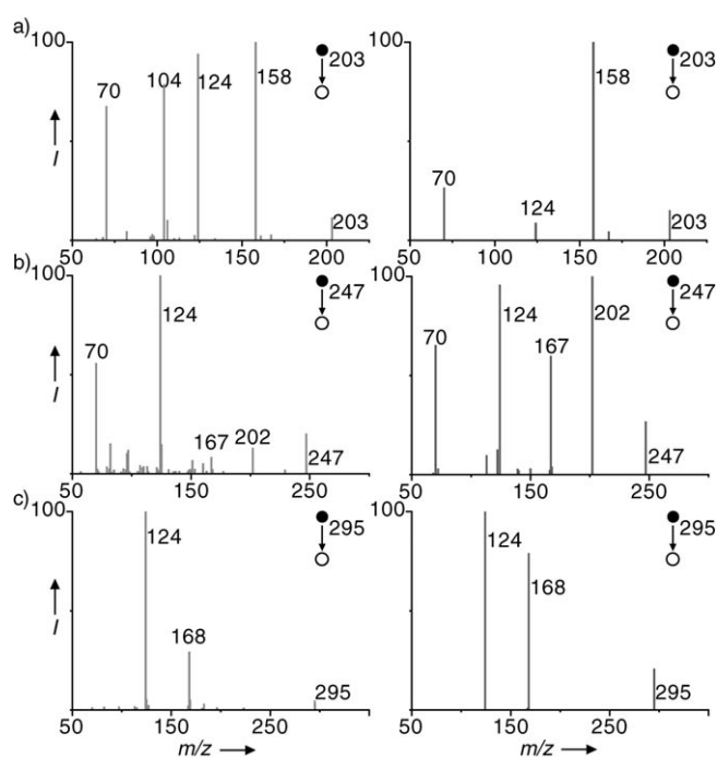
Figure 3. a) MS/MS spectra of the ion with m/z 203, which corresponds to T2 and/or 6 , at reaction times of milliseconds (left, dual ESI) and 1 s (right, microreactor). The fragment with m/z 104, which corresponds to C 4 H 7 NCl + , disappears with time. b) Same experiment but using NBS ( m/z 247). c) Same experiment but using NIS ( m/z 295).
