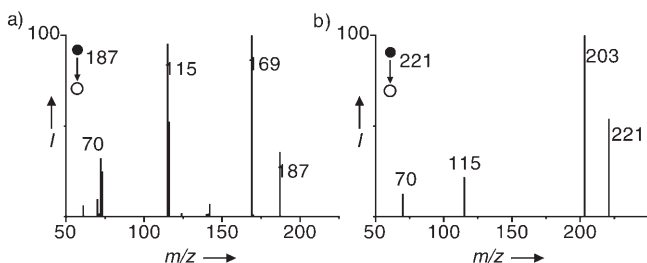
Figure 2. a) Dual ESI-MS/MS spectrum of T1 ( m/z 187). b) ESI-MS/MS spectrum of T3 ( m/z 221).
