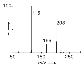
Figure 1. ESI-MS (positive mode) spectrum of the reaction after 30 minutes of 1 and NCS catalyzed by L-prolinamide.
